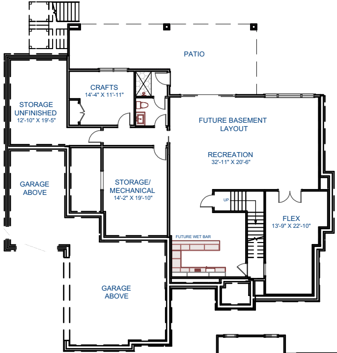
Future Basement
