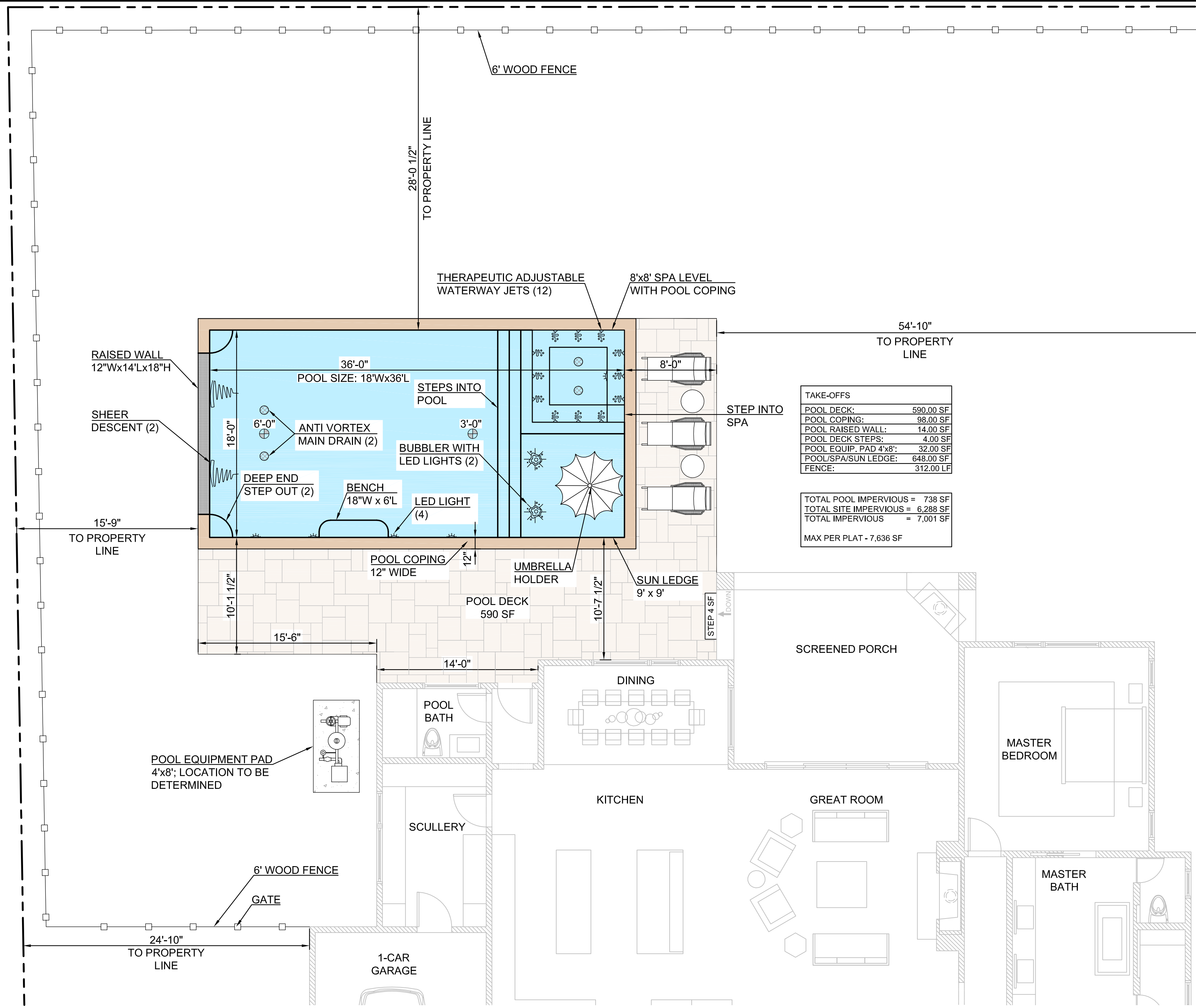
1 PRELIMINARY LUXURY POOL DESIGN SCALE: 3/16" = 1'-0"
